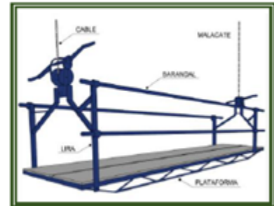
Hamaca
